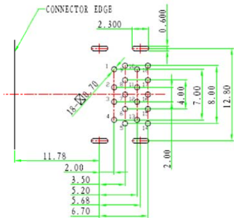
P.C.B. LAYOUT (COMPONENT SIDE) DEFAULT TOLERANCE: ± 0.05
